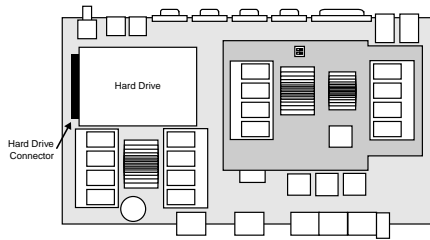
Figure 5: Drive Location on Fame CPU (4800AR-002)
