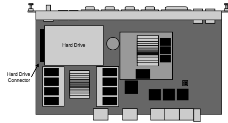
Figure 8: Drive Location on Frame CPU (4810AR-002)
