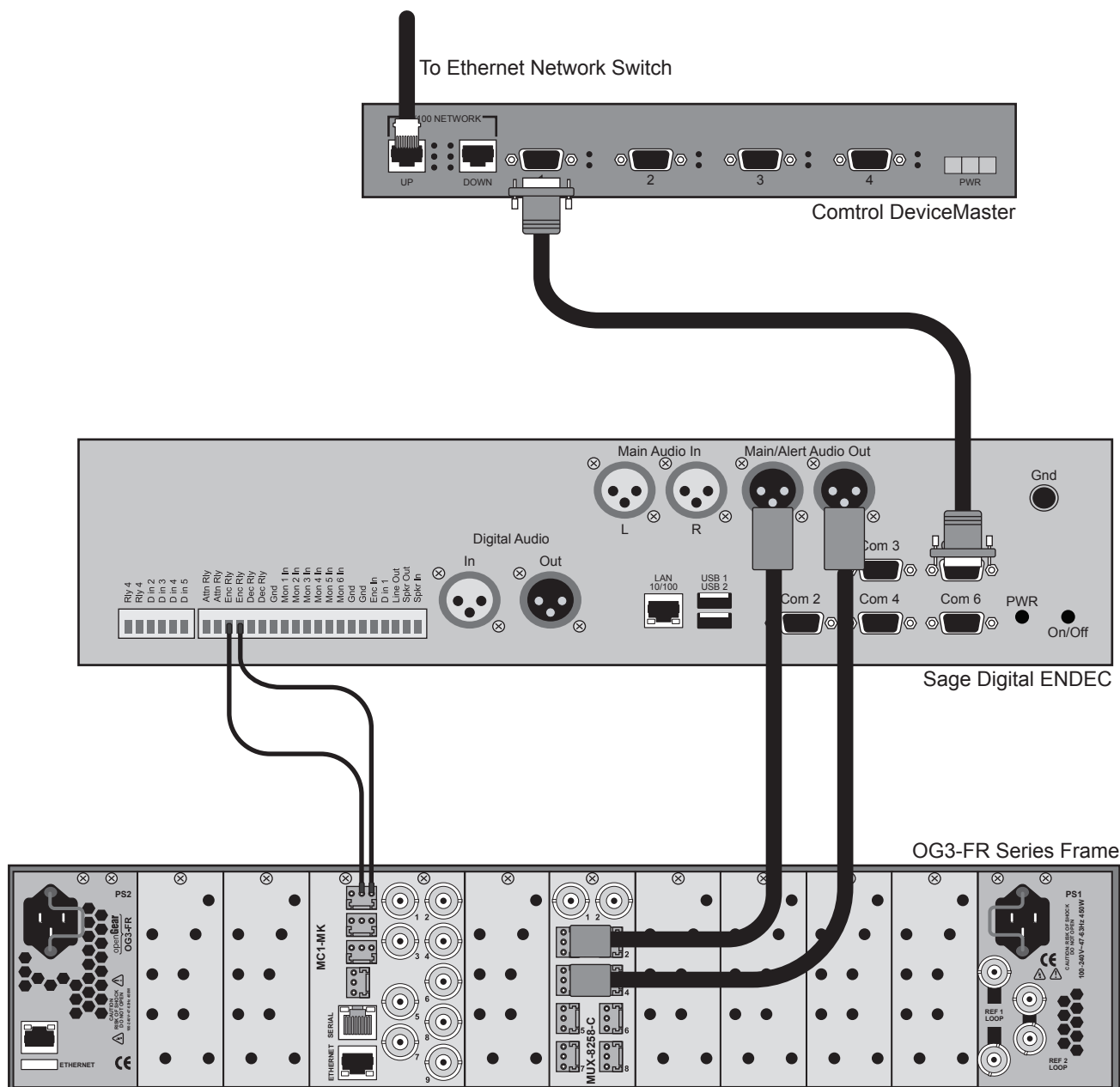
Figure 1 Cabling Designations
