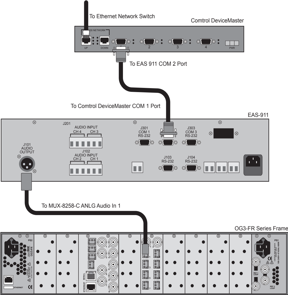
Figure 1 Cabling Designations
