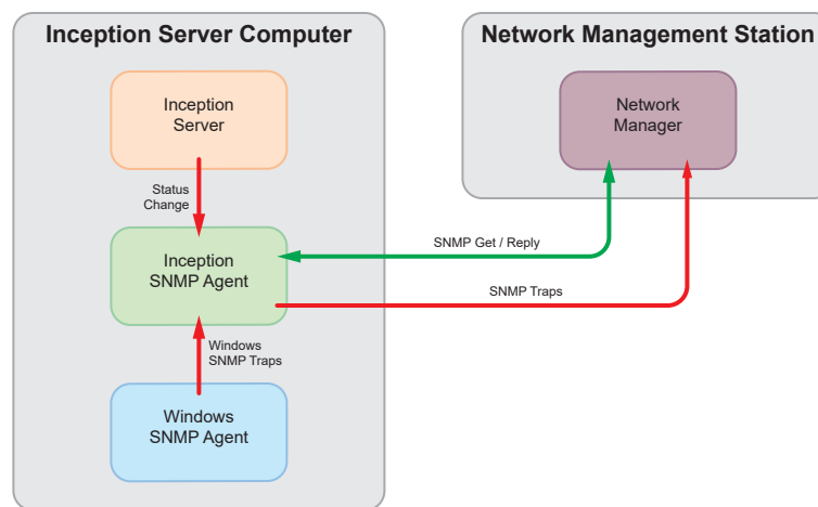
Figure 2.1 SNMP Connections
