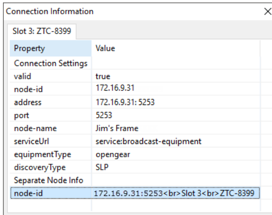
Figure 87 – Connection Settings
