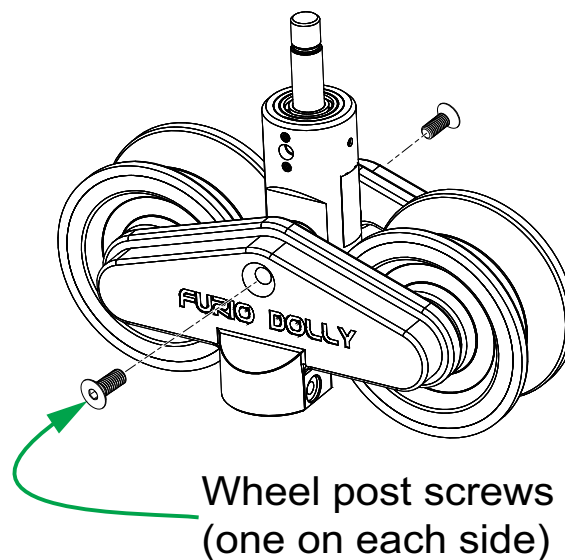
Figure 10 - Removing the Passive Wheel Post Screws
