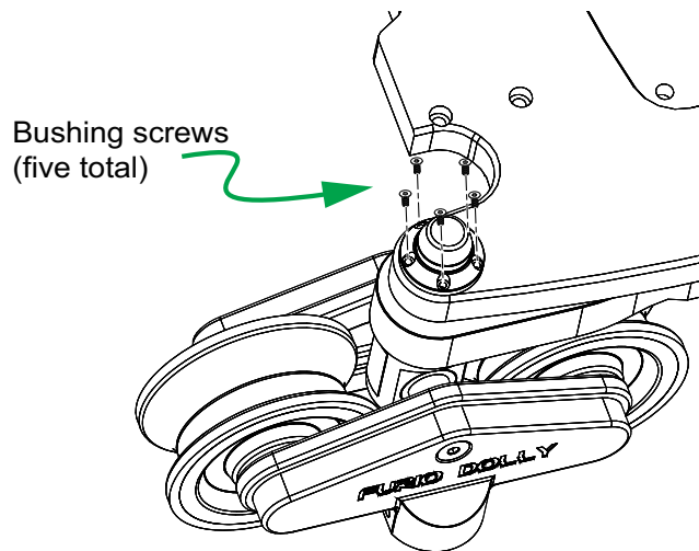
Figure 12 - Removing the Passive Wheel Bushing on the StableTrac Side
