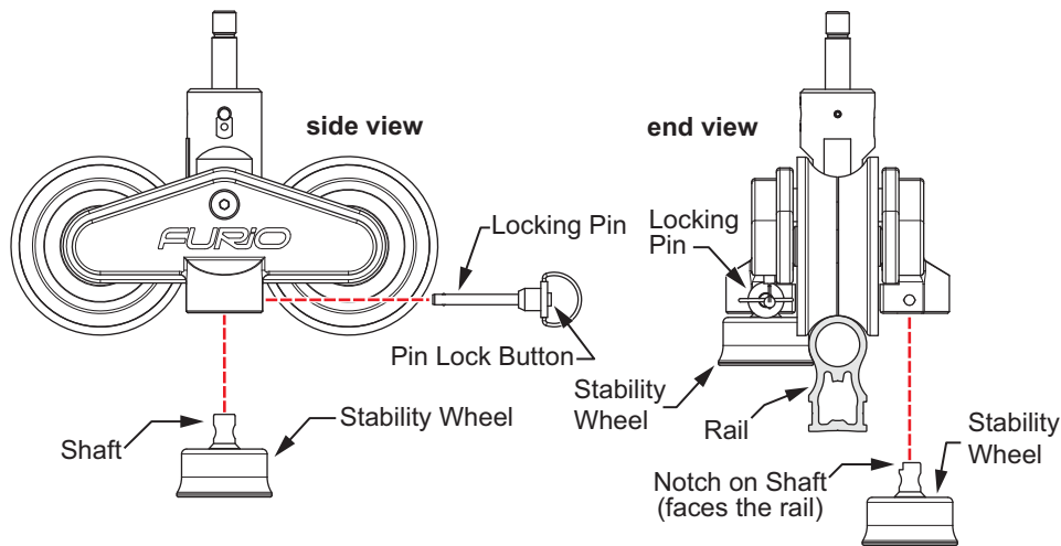
Figure 15 - Attaching Stability Wheels
