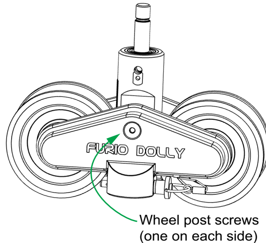
Figure 13 - Removing the Passive Wheel Post Screws
