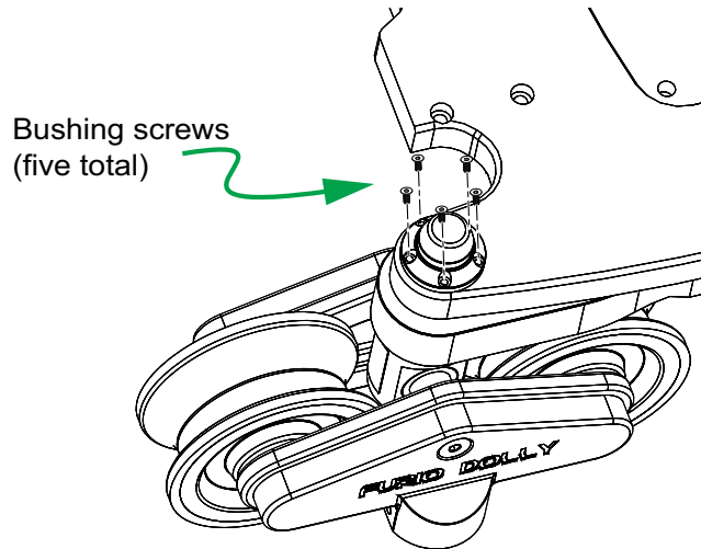
Figure 14 - Removing the Passive Wheel Bushing on the StableTrac Side
