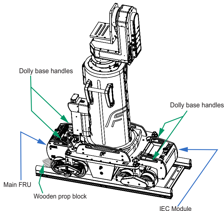
Figure 8 - Moving the Wooden Prop Block under the Main FRU
