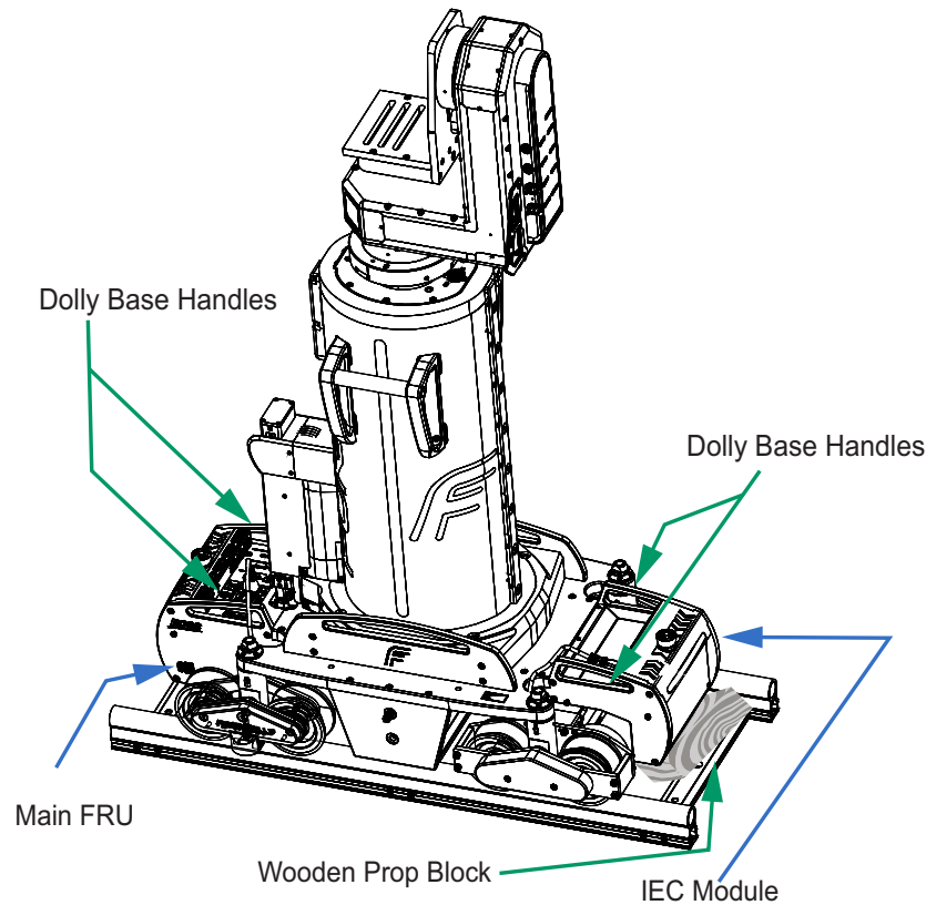
Figure 5 - Dolly Handles and Wooden Prop Block under the IEC Module
