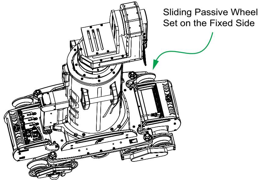
Figure 6 - Sliding Passive Wheel Set on the Fixed Side of the Dolly
