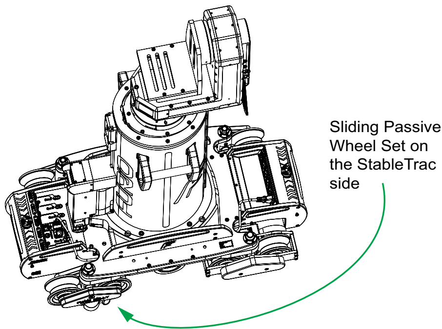
Figure 11 - Sliding Passive Wheel set on the StableTrac Side of the Dolly
