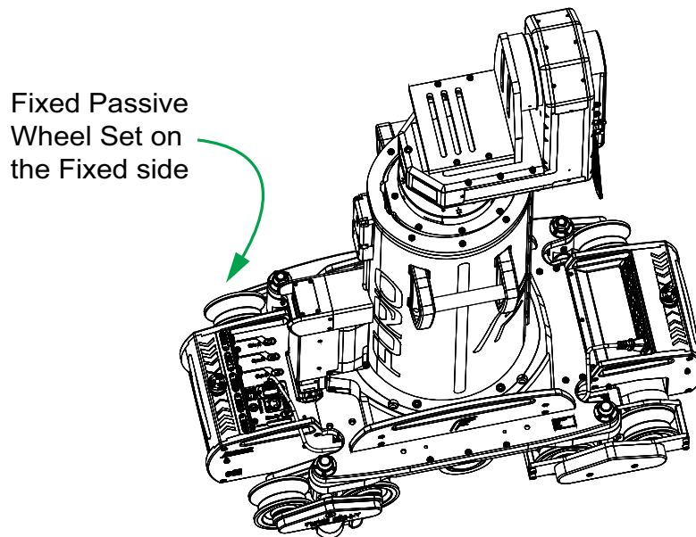
Figure 9 - Fixed Passive Wheel Set on the Fixed Side of the Dolly
