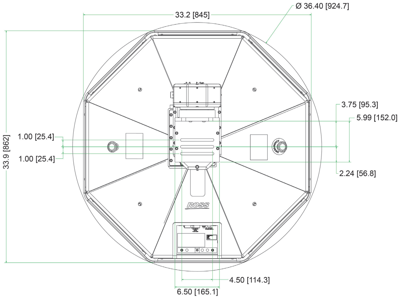
Figure 4 - CamBot 600XY-S3 Pedestal (top view)
