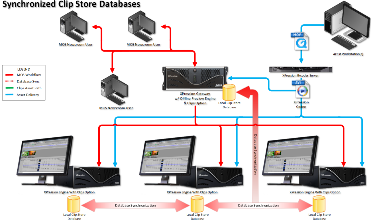
Clips Workflow Configuration when Using Multiple Workstations and Synchronized Clip Store Databases in a MOS workflow
