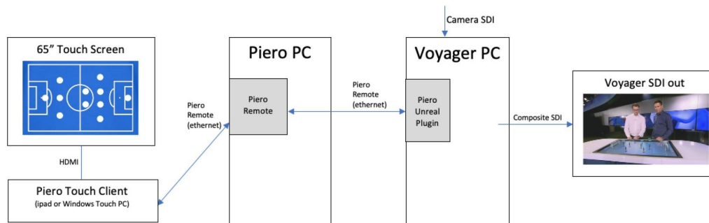
Hardware Schematic
