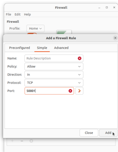
Add a Firewall Rule Dialog
