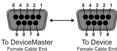
Serial Interface Cable (DB9 to DB9)
