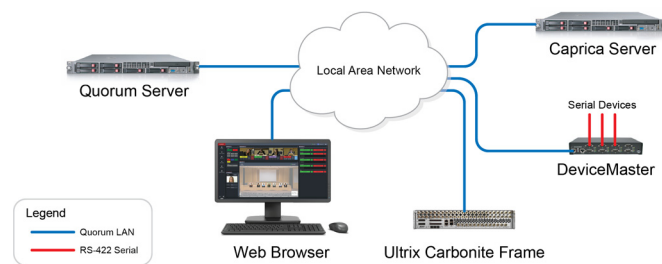
Figure 8.1 Quorum System Connection to an Ultrix Carbonite Switcher
