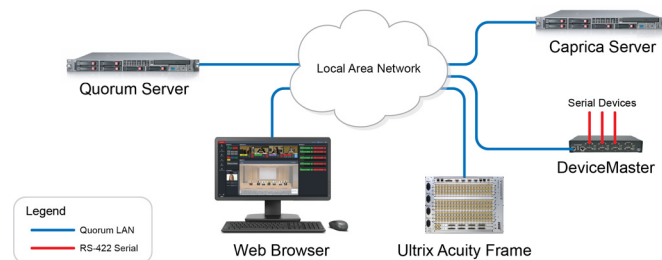
Figure 14.1 Quorum System Connection to an Ultrix Acuity Switcher
