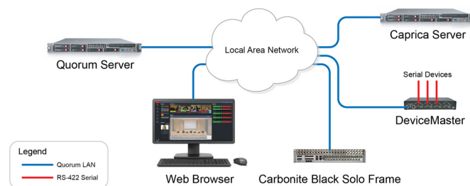
Figure 10.1 Quorum System Connection to a Carbonite Black Solo Switcher
