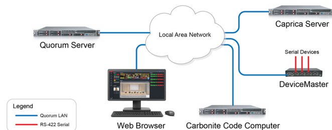
Figure 7.1 Quorum System Connection to a Carbonite Code Switcher
