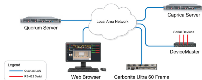
Figure 5.1 Quorum System Connection to a Carbonite Ultra 60 Switcher
