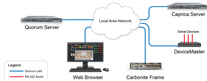
Figure 11.1 Quorum System Connection to a Carbonite Switcher
