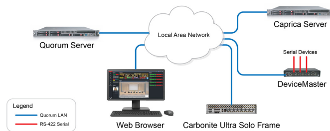
Figure 6.1 Quorum System Connection to a Carbonite Ultra Solo Switcher
