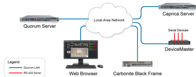
Figure 9.1 Quorum System Connection to a Carbonite Black Switcher
