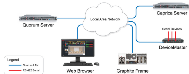
Figure 13.1 Quorum System Connection to a Ross Video Graphite All-In-One Production System
