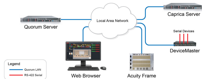
Figure 15.1 Quorum System Connection to an Acuity Switcher
