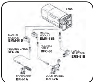
MM-21 Manual Focus/Manual Zoom
