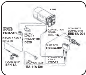
MS-22D (w/Shot Box) Manual Focus/Servo Zoom
