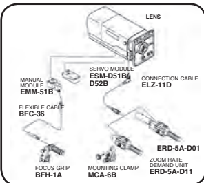
MS-21D Manual Focus/Servo Zoom
