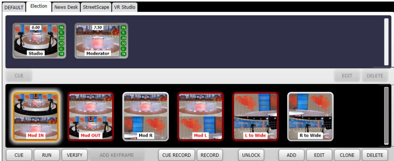
Figure 5 - Moves Panel
