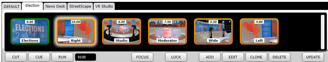
Figure 3 - Presets Panel
