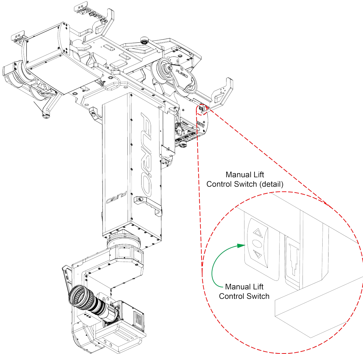
Figure 20 - SkyDolly, showing location of the Manual Lift Control Switch
