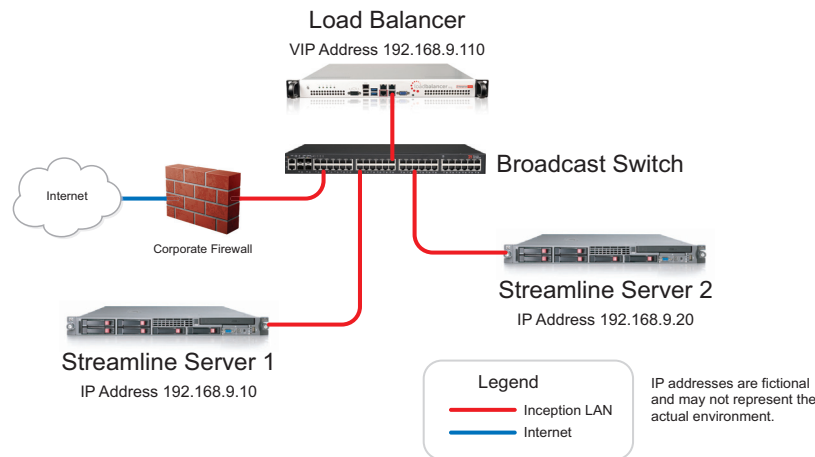
Figure 2.1 Streamline Redundant System
