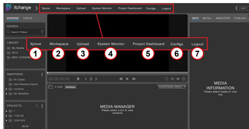
Figure 2.2 Main Screen
