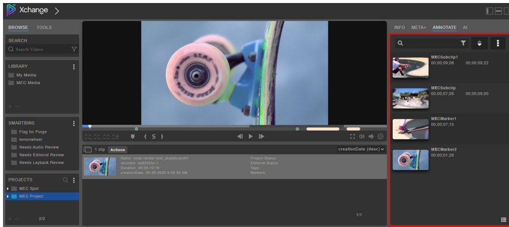
Figure 7.1 ANNOTATE Tab
