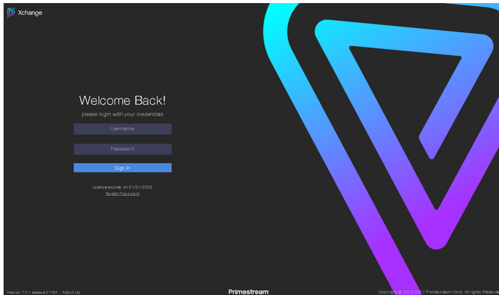
Figure 2.1 Login Screen
