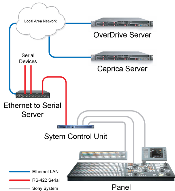
Sony MVS-8000G Switcher Cable Connections
