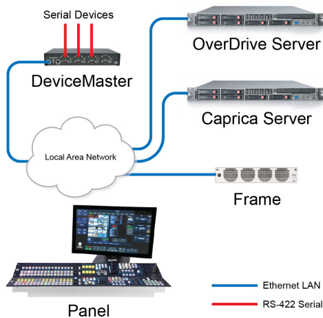
Snell Kula Switcher Cable Connections
