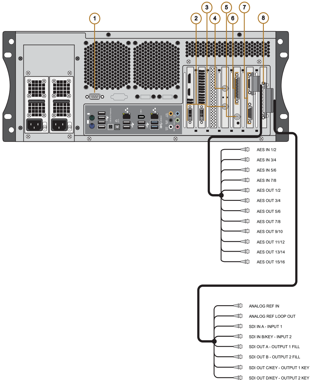
Figure 2.4 XPression Rear Input/Output Connections
