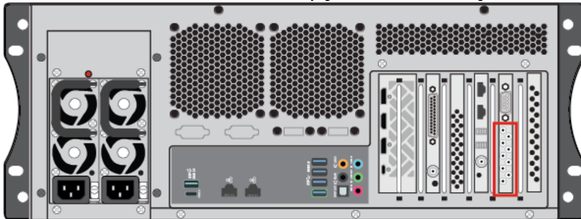
BNC Connections
