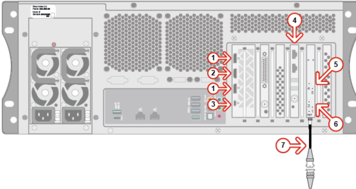
Voyager 12G Rear Input/Output Connections
