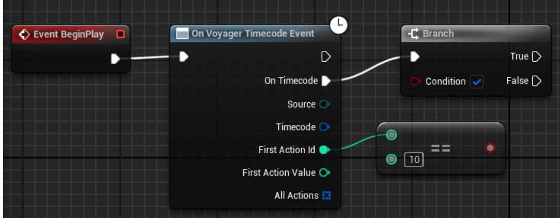
On Voyager Timecode Event - Branch Node Added
