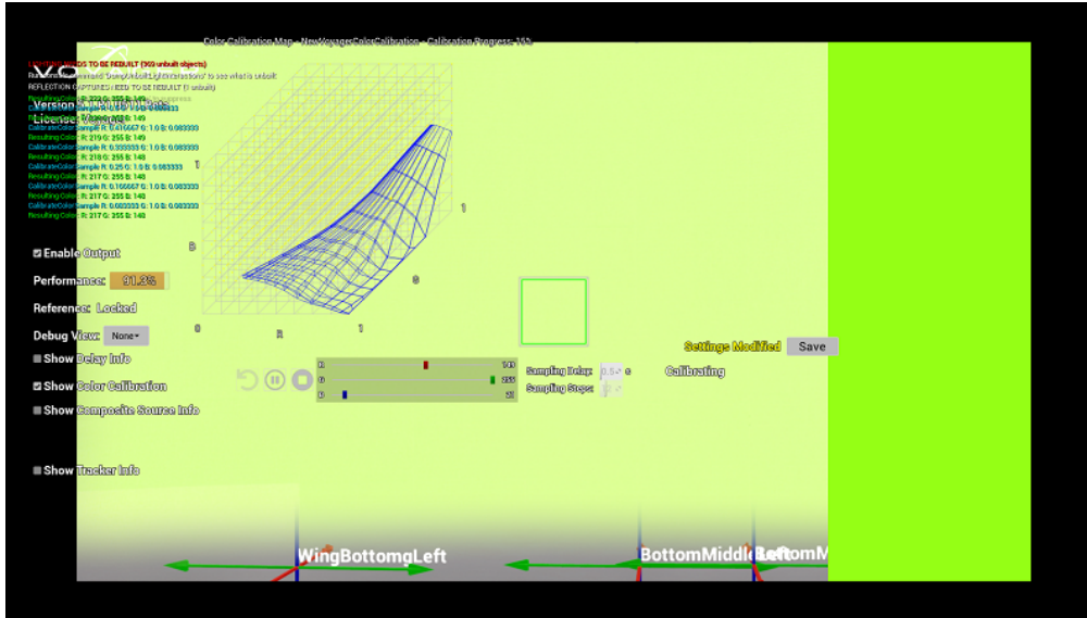
Color Sampling
