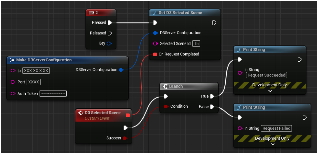
Set D3 Selected Scene Blueprint
