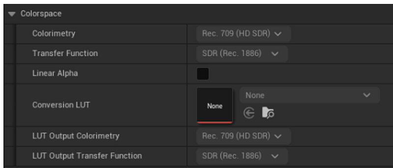
Colorspace Settings
