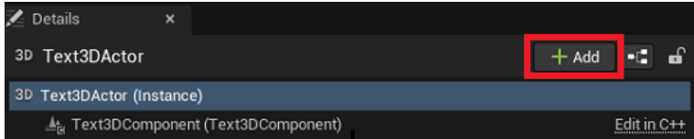
Add Component
