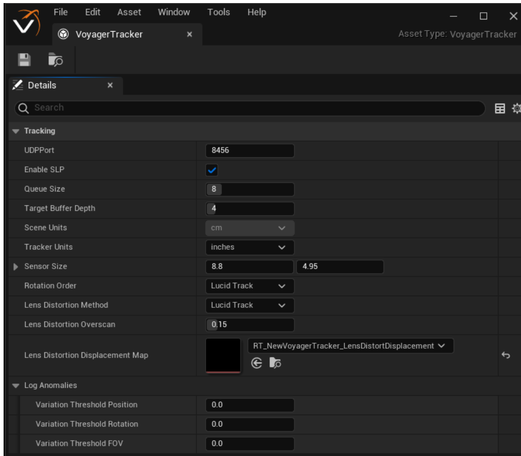
VoyagerTracker - Details
