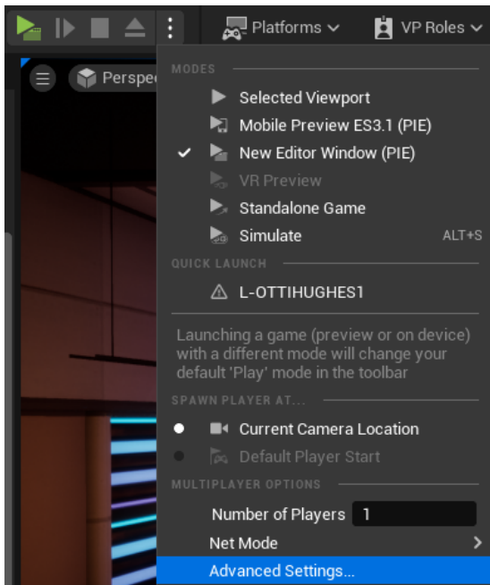
Advanced Settings
