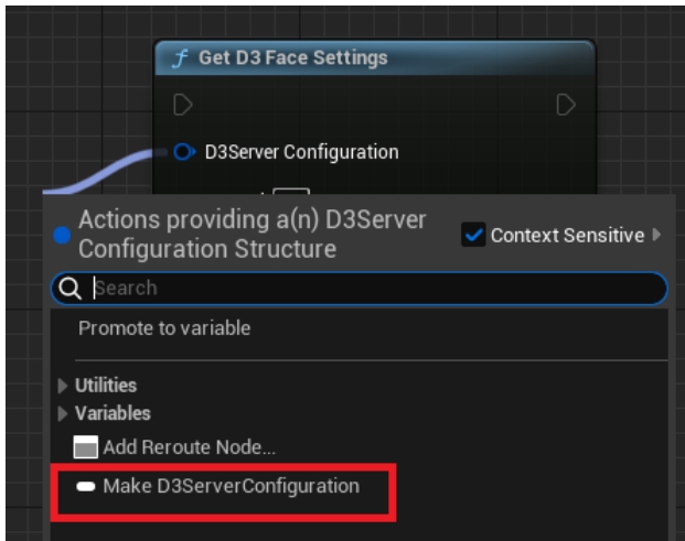
Make D3ServerConfiguration
