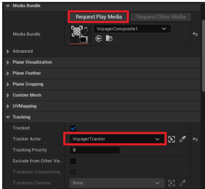
Configure VoyagerComposite1
