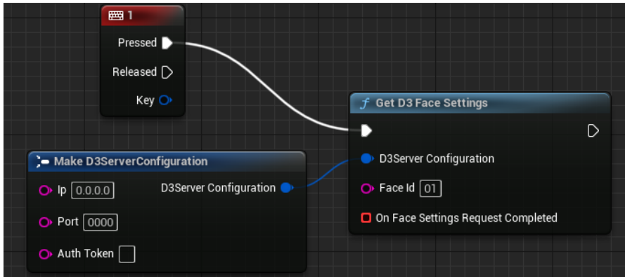
Add Trigger
