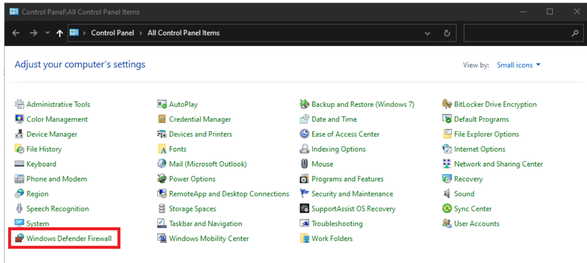
Control Panel
