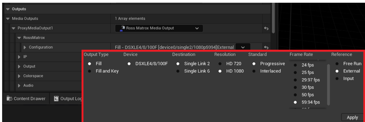
Output Configuration
