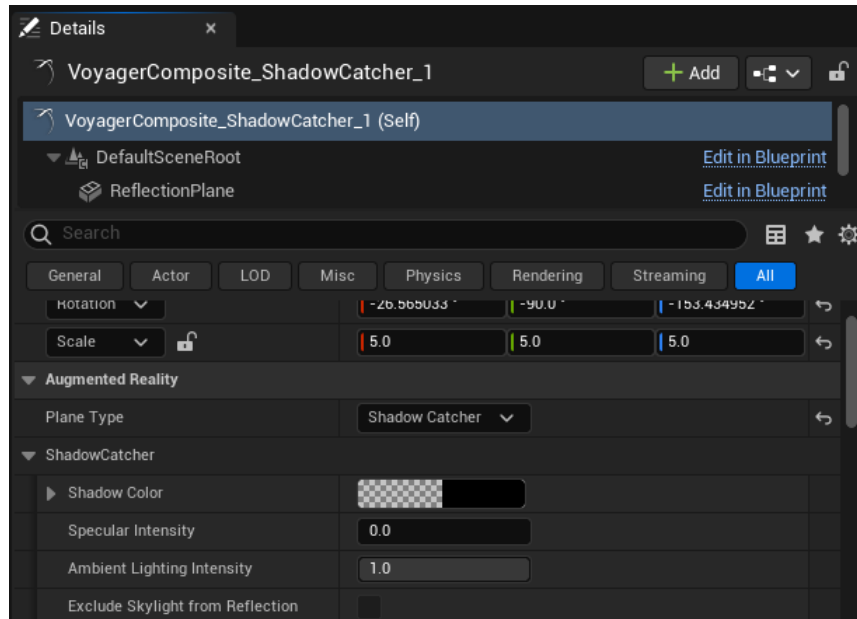
VoyagerComposite_ShadowCatcher
