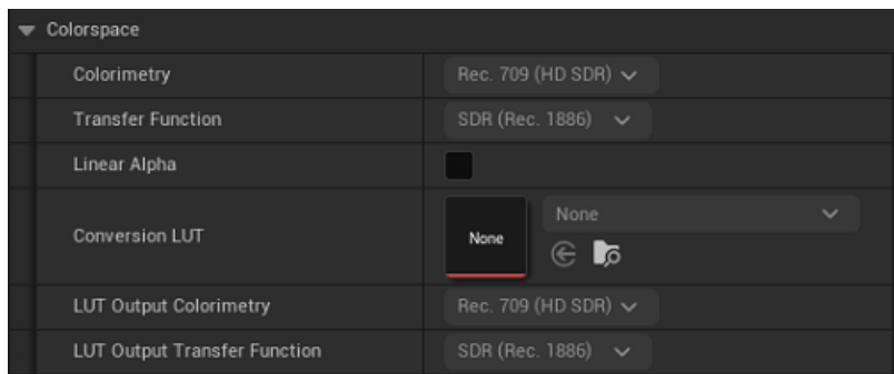
Colorspace Settings
