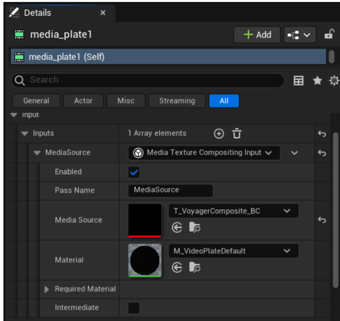
Media_plate1 Details
